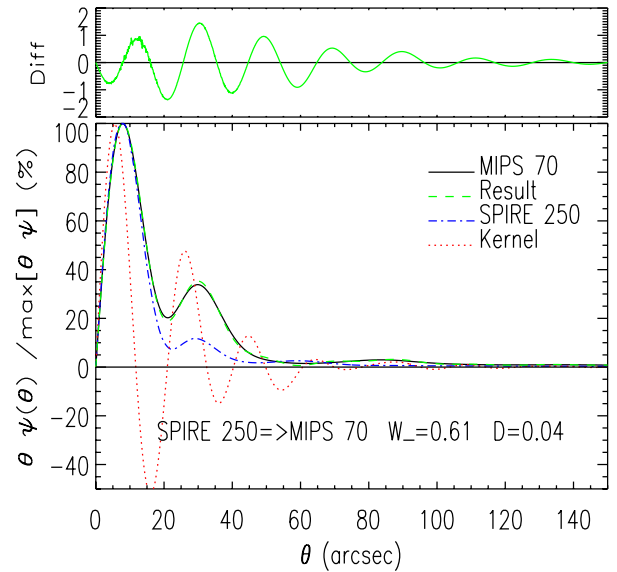
FIG. 5.—Performance of the kernel K\{S250 \Rightarrow M70\} . With W_- = 0.61 , this kernel is safe to use. \Psi_{S250} \star K\{S250 \Rightarrow M70\} deviates from \Psi_{M70} less than 2%. See the electronic edition of the PASP for a color version of this figure.
