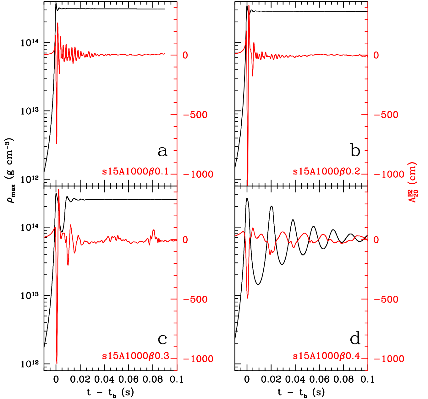
FIG. 8.— Maximum density ( \rho_{max} , black) and gravitational wave amplitude ( A_{20}^{E2} , red) as functions of time for the Woosley and Weaver (1995) s15 model and A = 1000 km. For each model, the zero of the time axis is set to the time of core bounce ( t_b ). a (upper left): \beta_i=0.10\% , bounce at supranuclear density with negligible influence of centrifugal forces (type I). Note the subsequent ring-down waveform, which is associated with both radial- and non-radial modes of the compact remnant. b (upper right): \beta_i=0.20\% , similar to the previous model, but with greater asphericity leading to larger amplitudes. c (lower left): Transitional model with \beta_i=0.30\% , which is beyond the \beta_i for the largest gravitational wave amplitudes. The typical oscillation period of the waveform is significantly larger than those of the previous models and the hydrodynamic data exhibit at least one additional coherent large scale expansion-collapse-bounce cycle caused by the growing influence of centrifugal forces. d (lower right): \beta_i=0.40\% . The hydrodynamic evolution and the associated waveform of this model are already largely influenced by centrifugal forces. The core exhibits subsequent multiple coherent bounces that are quasi-exponentially damped (type II).
