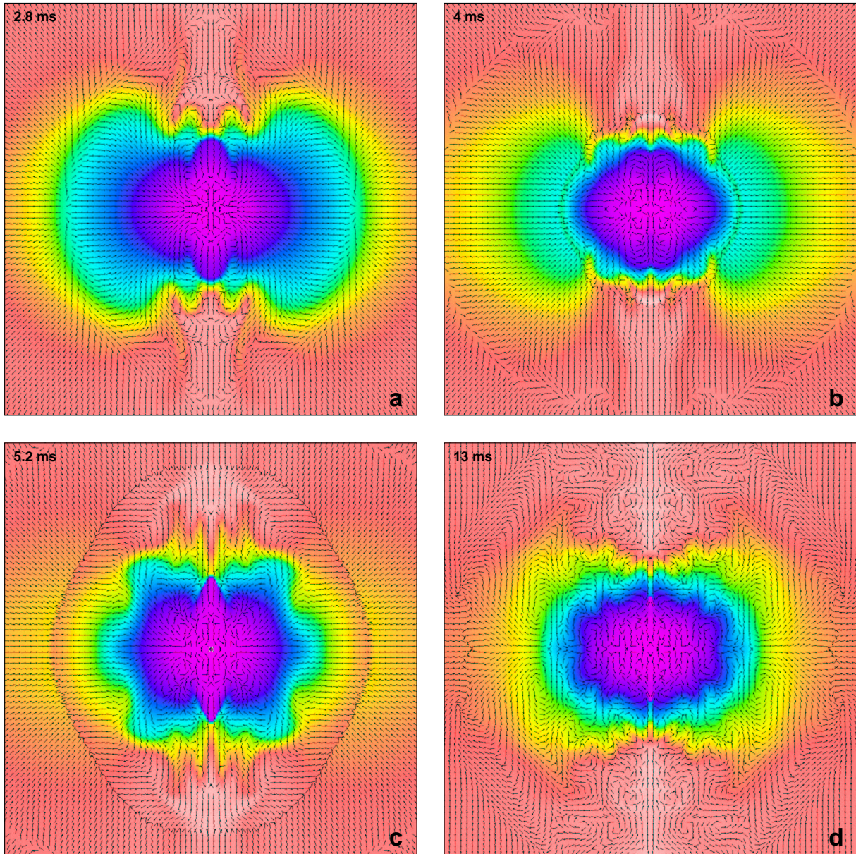
FIG. 5.— 2-D plots of the specific entropy of the inner 200 \times 200 \text{ km}^2 of the s15A1000/30.2 model depicting the ring-down epoch of the evolution of this generic type I model. The color map goes from light red for high specific entropy ( s=16 \text{ k}_B ) to magenta for low entropy ( s=0.7 \text{ k}_B ). The times given in the top left-hand corners are the snapshot times after bounce. Velocity vectors for the r and \theta motions (not the \phi motion in the angular direction) are superposed. As the core executes successive radial and non-radial post-bounce oscillations, it generates strong sound waves (weak shock waves) that are seen in panels (b) and (c) as contours of velocity discontinuity. At the time of panel (a), the actual bounce shock has already left the frame. Panel (d) shows the compact remnant at 13 ms after bounce when it has already lost most of its excess pulsational energy. The velocities at that time are dominated by incoherent vortical motions. (This figure is available in high-quality format from http://www.ita.uni-heidelberg.de/~cott/gwpaper .)
