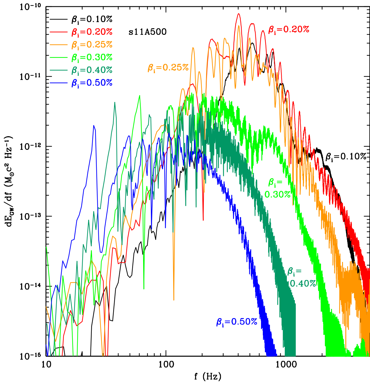
FIG. 21.— Same as Fig. 10, but for the s11A500 sequence and for \beta_i s from 0.1% to 0.5%.
