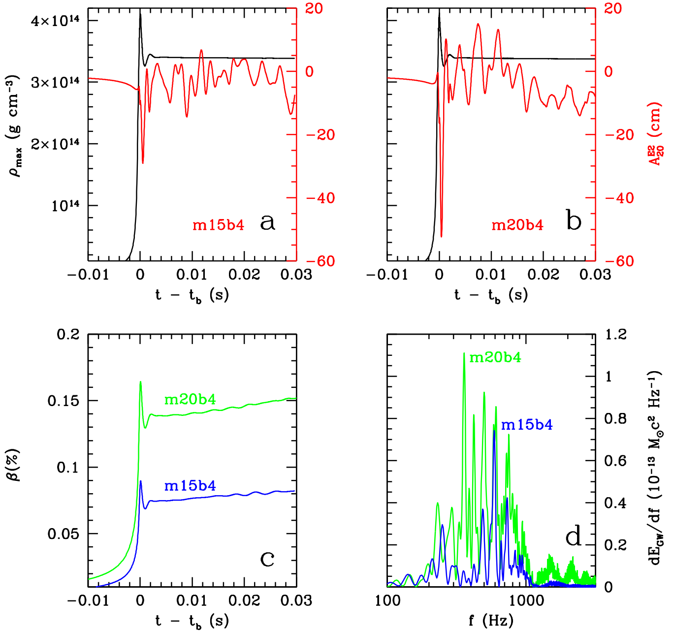
FIG. 17.— The 15 and 20 M_{\odot} models from Heger et al. (2003). a (upper left): Evolution of the maximum density (black) and the gravitational wave amplitude (red) of the m15b4 model. b (upper right): The same for the m20b4 model. Both models rotate very slowly and rigidly and show only small deviations from spherical symmetry. Hence, the gravitational wave amplitudes are small. c (lower left): This figure depicts the evolution of the rotation parameter \beta for these models. Both models bounce due to the stiffening of the equation of state at nuclear density, with little contribution due to centrifugal forces. The model with the greater \beta , m20b4, reaches a larger final \beta . d (lower right): Energy spectra. The spectrum of the m20b4 model peaks at lower frequencies and contains significantly more energy (4 times more; see Table 6) than the spectrum of the m15b4 model. This shows the sensitivity of the gravitational wave signature to small differences in the initial rotation profile and stellar structure.
