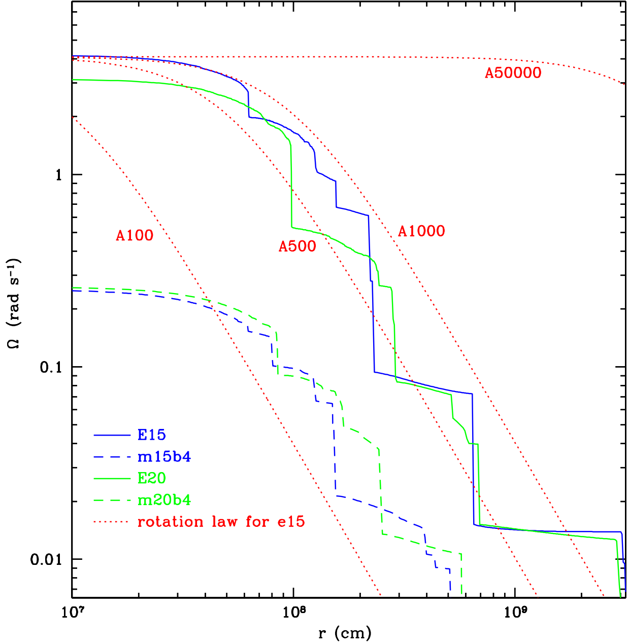
FIG. 3.— Initial angular velocity profiles of the rotating 15 (blue) and 20 (green) M_{\odot} progenitor models (see Table 1 for model parameters). The dotted red profiles were generated with the rotation law of eq. (5) using the central \Omega of model e15 for \Omega_0 . All realistic presupernova models exhibit near rigid rotation inside \simeq 1000 km. Note the much smaller angular velocities exhibited by models m15b4 and m20b4, which were evolved with the inclusion of magnetic fields.
