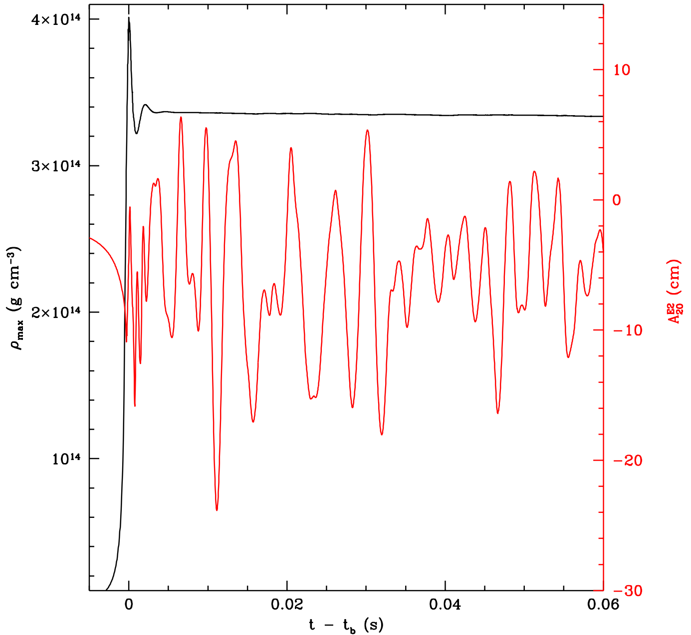
FIG. 18.— Evolution of the maximum density (black) and the gravitational wave amplitude (red) of a s15 model evolved without rotation. The time is given relative to the time of core bounce. Small scale perturbations, introduced by the finite-difference approximation and post-bounce convective instability, lead to continuous gravitational wave emission with amplitudes that are one to two orders of magnitude smaller than those observed from the collapse of a rotating model.
