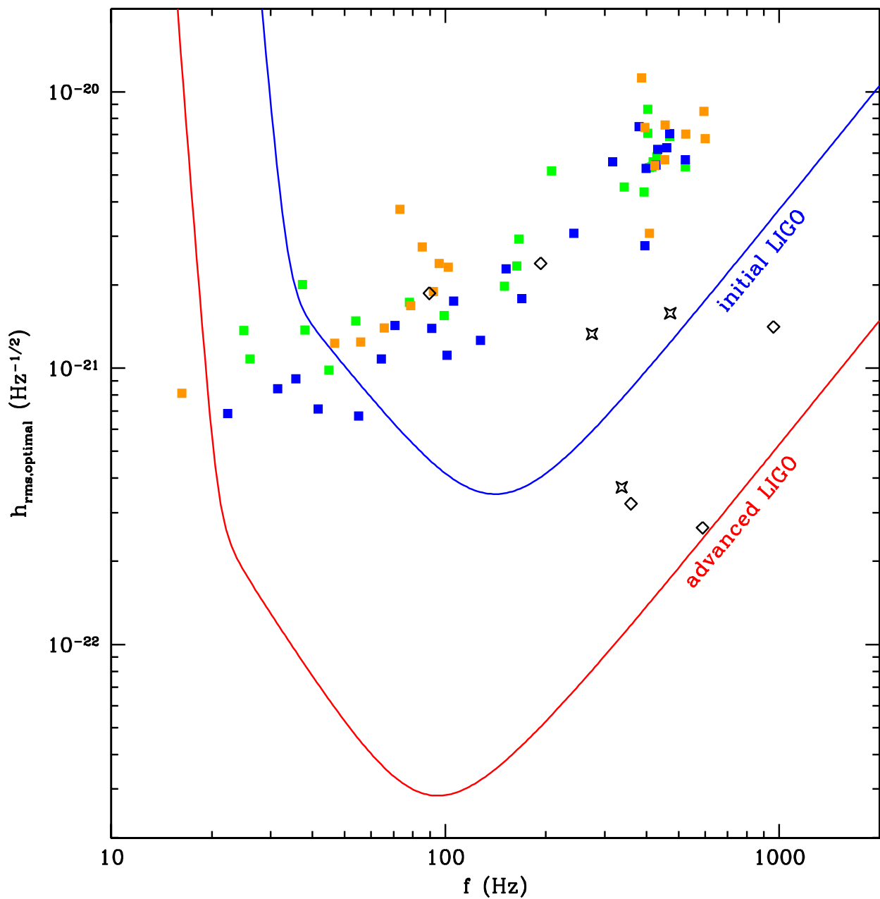
FIG. 20.— LIGO sensitivity plot. Plotted are the optimal root-mean-square noise strain amplitudes h_{rms} = \sqrt{fS(f)} of the initial and advanced LIGO interferometer designs. Optimal means that the gravitational waves are incident at an optimal angle and optimal polarization for detection and that there are coincident measurements of gravitational waves by multiple detectors. For gravitational waves from burst sources incident at random times from a random direction and a signal-to-noise ratio (SNR) of 5, the rms noise level h_{rms} is approximately a factor of 11 above the one plotted here (Abramovici et al. 1992; Flanagan and Hughes 1998). We have plotted solid squares at the maxima of the characteristic gravitational wave strain spectrum ( h_{char}(f) ; §8) of our s11 (green), s15 (blue), and s20 (orange) models from Woosley and Weaver (1995) that were artificially put into rotation. Our nonrotating models are marked with stars; diamonds stand for models from Heger, Langer, and Woosley (2000) and Heger et al. (2003). The distance to Earth was set to 10 kpc for all models. Most of our models lie above the optimal design sensitivity limit of LIGO I. Hence, the prospects for detection are good. Those models that are not detectable by the 1st-generation LIGO are those that rotate most slowly (the Heger et al. 2003 models) and those which are the fastest rotators.
