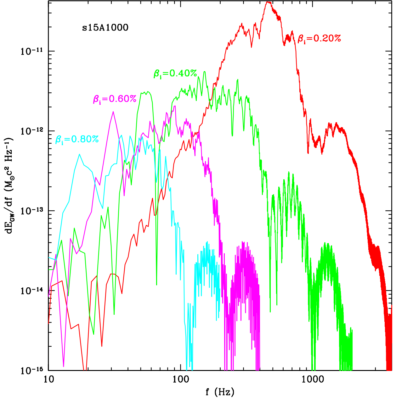
FIG. 10.— Energy spectra of the gravitational radiation emitted from representative models of the s15A1000 model series. Note the shift of the spectra to lower frequencies with increasing \beta_i and the logarithmic scale of the ordinate. The spectra have been cut off at a frequency beyond which generic high frequency noise at constant magnitude sets in. The first pronounced peak in the spectra of the more strongly rotating models can be identified with the frequency of the expansion-collapse-bounce cycles exhibited by these models (type II). The spectra of the slower rotators peak at the dominant frequencies of the post-bounce ringing of the compact remnant. The higher harmonics are clearly seen in these models.
