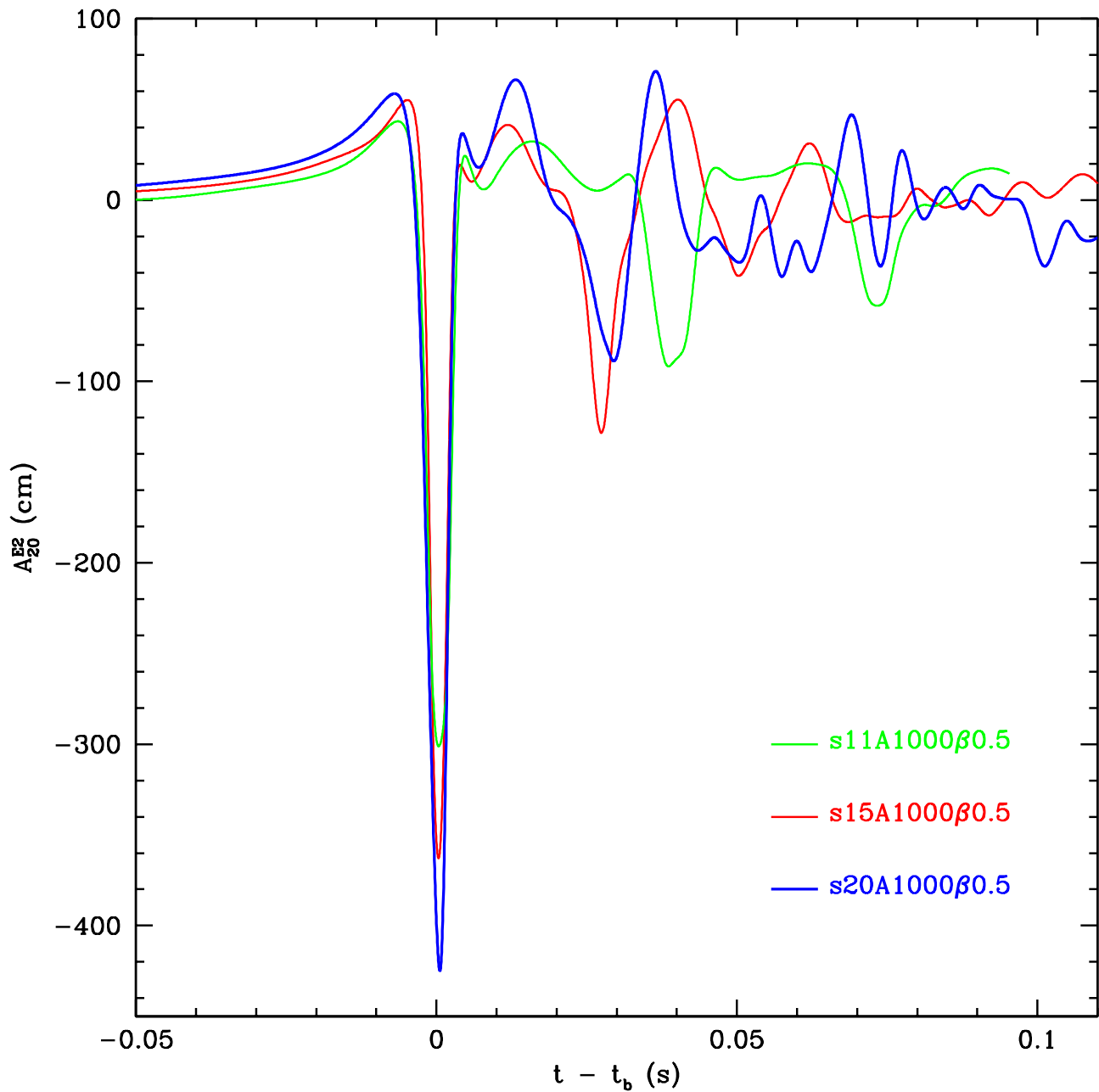
FIG. 14.— Comparison of the evolution of the gravitational wave signal A_{20}^{E2}(t) of models s11, s15 and s20 for A=1000 km and \beta_i=0.50\% . The waveforms reflect the density evolution seen in Fig. 12. For the s20 signal, additional high-frequency contributions appear to be correlated with the vortical motions and aspherical infall seen behind its stalled shock.
