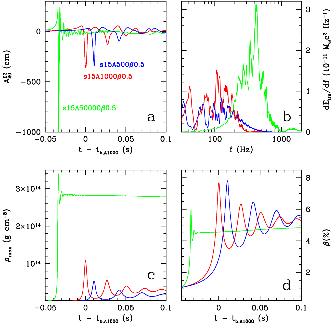
FIG. 11.— Comparison between different initial distributions of angular momentum at fixed \beta=0.50\% for the s15 model from Woosley and Weaver (1995). Models A50000, A1000, and A500 are nearly rigidly rotating interior to 50000, 1000, and 500 kilometers, respectively. a (upper left): Time evolution of the gravitational wave amplitude for the models s15A50000 \beta .5, s15A1000 \beta .5, and s15A500 \beta .5. The time axis is relative to the time of bounce of the s15A1000 \beta .5 model. For a given model the transition from a bounce dominated by nuclear repulsive forces to one in which centrifugal forces play a significant role occurs at progressively lower \beta_i with decreasing A. b (upper right): Energy spectra of the three models. Note the distinct peak of the rigidly rotating s15A50000 \beta .5 model (green) at about 400 Hz that is directly associated with the post-bounce ringing of the compact remnant, also seen in the waveform. The spectra of the models with smaller A exhibit a local maximum at low frequencies that also directly correspond to the frequencies of their post-bounce expansion-collapse-bounce cycles. c (lower left): Evolution of the maximum density. Model s15A50000 \beta .5 still bounces at supranuclear densities, while the two models with smaller A have already made the transition to type II behavior. d (lower right): Evolution of the rotation parameter \beta with the time given relative to the time of bounce of model s15A1000 \beta .5. The models with A=1000 and A=500 have more angular momentum in their central regions and, hence, are more strongly influenced by centrifugal forces. For a given \beta_i , they also achieve larger final \beta_s and \beta_b s at bounce.
