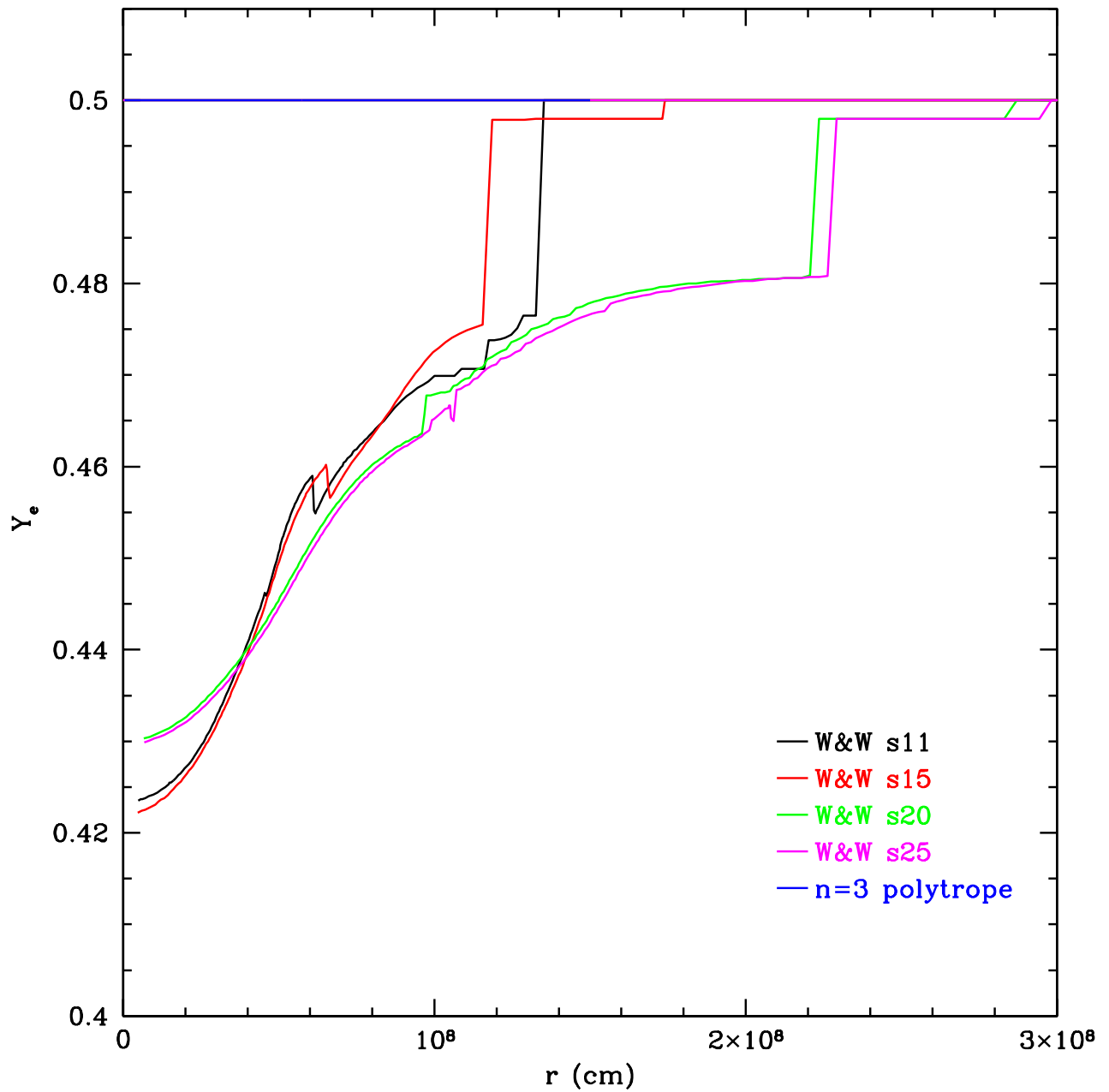
FIG. 2.— Electron number fraction Y_e as a function of radius for the Woosley and Weaver (1995) progenitor models. The central iron core has been neutronized due to electron capture during core silicon burning (Weaver, Zimmerman, and Woosley 1978). For the polytrope, Y_e has been assumed to be 0.5 (Zwinger and Müller 1997). The discontinuity in Y_e exhibited in the Woosley and Weaver models indicates the approximate boundary between the central iron core and the surrounding shells.
