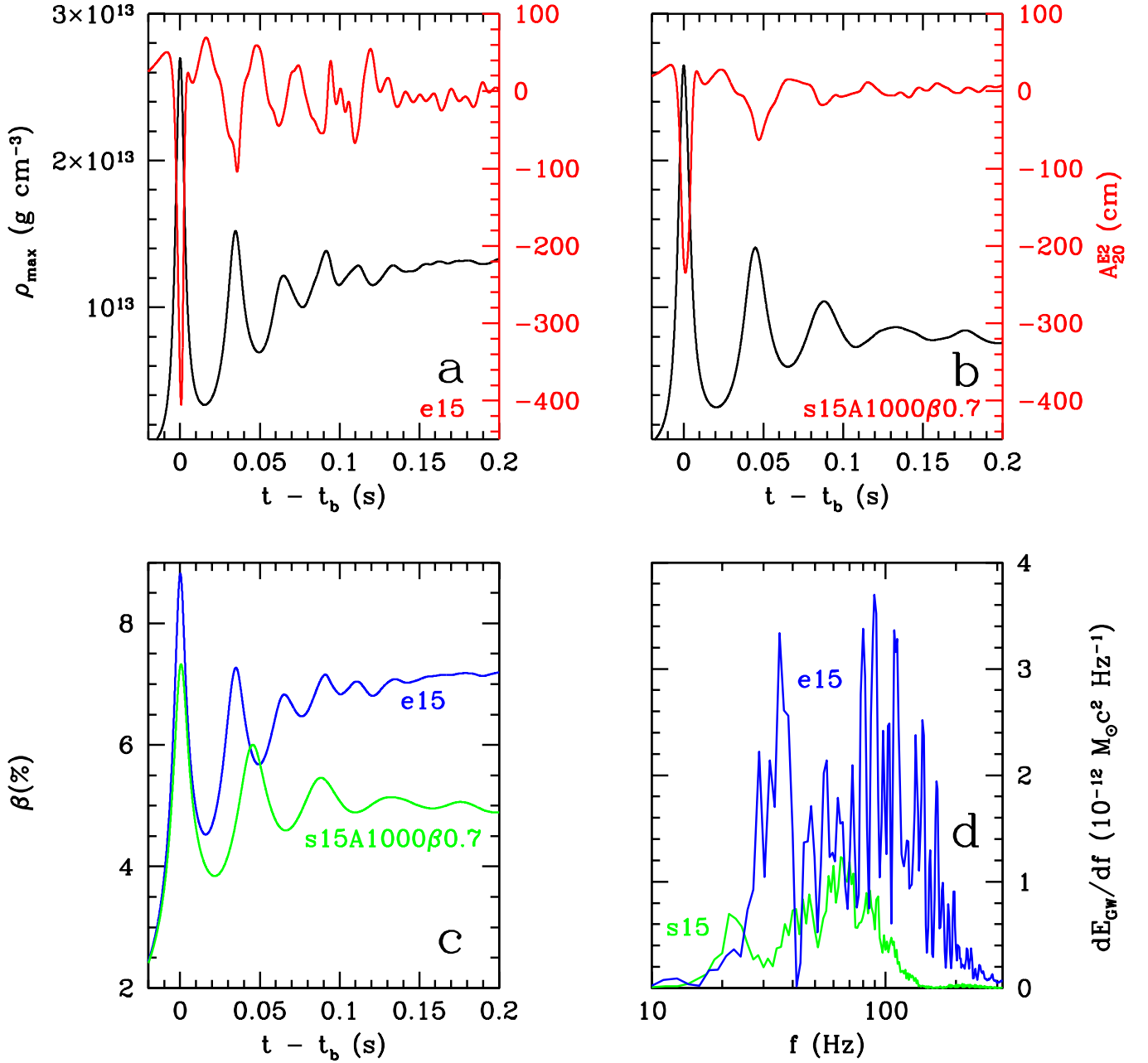
FIG. 16.— Comparison of the e15 model from Heger, Langer, and Woosley (2000) with the s15A1000 \beta 0.7 model from Woosley and Weaver (1995). Both models have similar initial \beta_i (0.645% for the e15 model versus 0.70% for the s15A1000 \beta 0.7 model) and angular velocity ( \Omega ) profiles but differ significantly in their total angular momenta. This is due to differences in their initial density profiles. a (upper left) and b (upper right) : Evolution of the maximum density and the gravitational wave amplitude, respectively, for models e15 and s15A1000 \beta 0.7. The waveform of e15 exhibits additional high-frequency components about 100 ms after bounce that we associated with the sudden damping of the post-bounce expansion-collapse-bounce cycles by infalling matter. This is also reflected in the evolution of the maximum density. c (lower left) : Evolution of the rotation parameter \beta for the two models. The larger angular momentum of model e15 and its specific distribution translate into a larger final \beta . d (lower right) : Energy spectra for the two models under consideration. The e15 model radiates significantly more energy and has distinctly more fine spectral structure.
