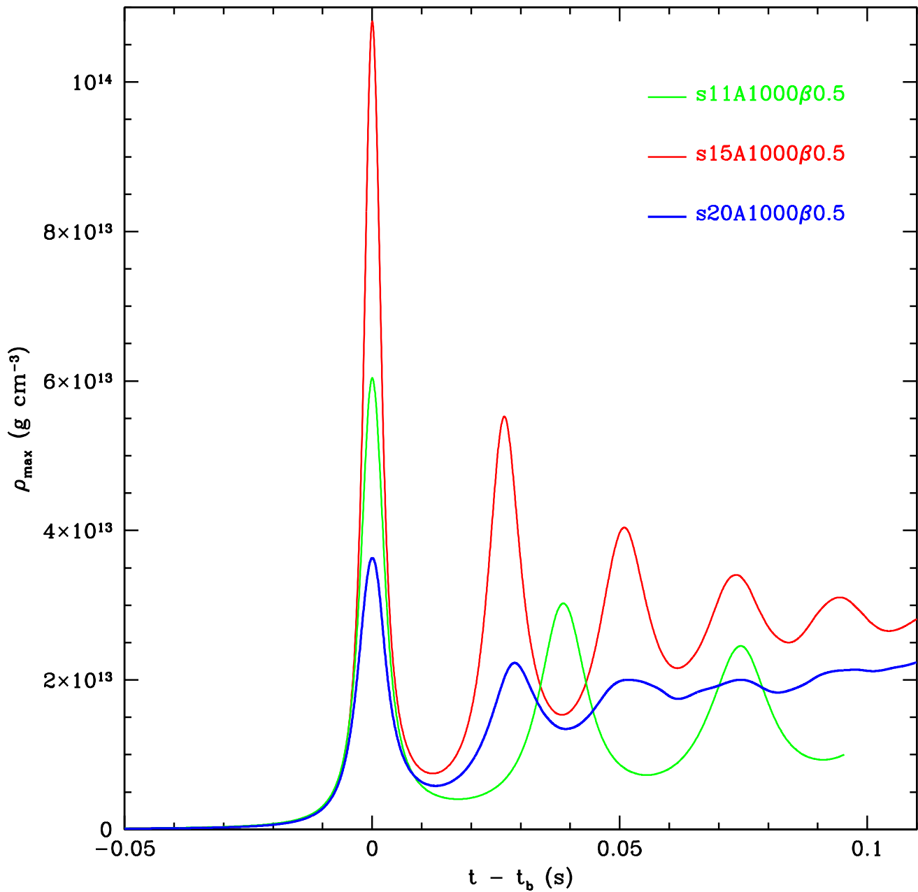
FIG. 12.— Inter-model comparison between s11A1000, s15A1000 and s20A1000 for \beta_i=0.50\% of the evolution of the peak density. The time is given relative to the time of bounce for each individual model. Model s15 reaches higher maximum densities and has the shortest post-bounce oscillation periods. Model s11, which has a similar initial density and angular momentum distribution, reaches lower densities and has longer post-bounce oscillation periods. The s20A1000 model, however, with significantly different initial density, angular momentum, and compositional profiles, bounces for the same A and \beta_i at even lower densities. It also has shorter oscillation periods than the s11 model and is more quickly damped by the proximity of its stalled shock.
