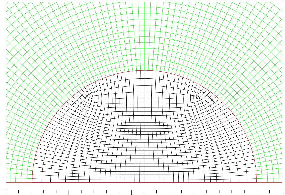
FIG. 4.— Central region of the VULCAN/2D computational grid. Shown in black is the inner 10 km, where the capability of VULCAN/2D to work with arbitrary grid configurations has been used to perform a smooth transition from the outer radial grid to a Cartesian grid in the innermost region.
