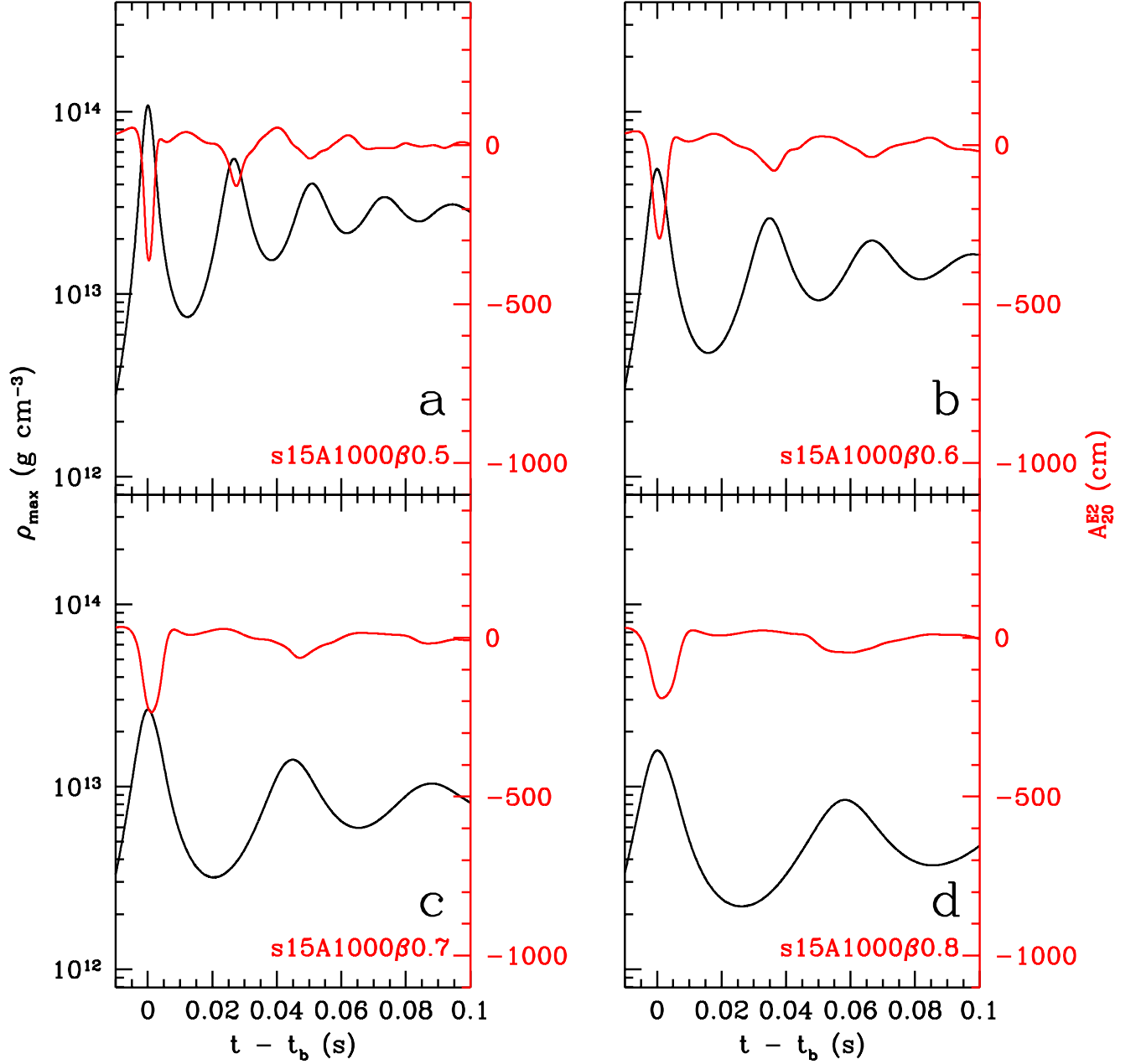
FIG. 9.— Same as Figure 8, but for higher values of \beta_i . \rho_{\max}(t) (black) is the maximum density and A_{20}^{E2}(t) (red) is the gravitational wave amplitude for s15A1000. a (upper left): This model with \beta_i=0.50\% undergoes a bounce at subnuclear density when centrifugal forces overcome gravitational attraction. Note the significantly larger dynamical timescales compared with models with smaller \beta_i . Panels b, c and d: As \beta_i increases from 0.60% to 0.80%, bounce occurs more slowly and at progressively lower densities. The waveforms are dominated by the subsequent expansion-collapse-bounce cycles of the quickly spinning deformed stellar core (type II).
