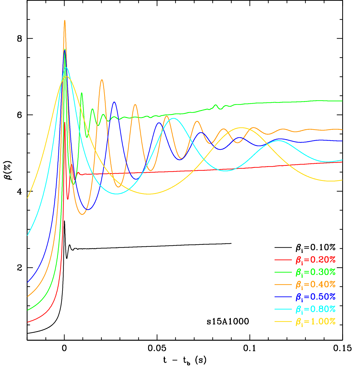
FIG. 7.— Evolution of the ratio of rotational to gravitational energy (rotation parameter \beta ) for the s15A1000 model series. The zero of the time axis is set to the time of bounce for each model. The \beta_i=0.40\% model, which is the first to bounce by centrifugal forces, reaches the maximum \beta at bounce for all models. The \beta_i=0.30\% model has a smaller \beta at bounce but shows, due to the greater compactness of its remnant, the largest final \beta . The models with \beta_i > 0.40\% collapse so slowly that centrifugal forces are able to halt collapse before greater compression can lead to very large \beta s. None of our models exceeds a \beta of 10%.
