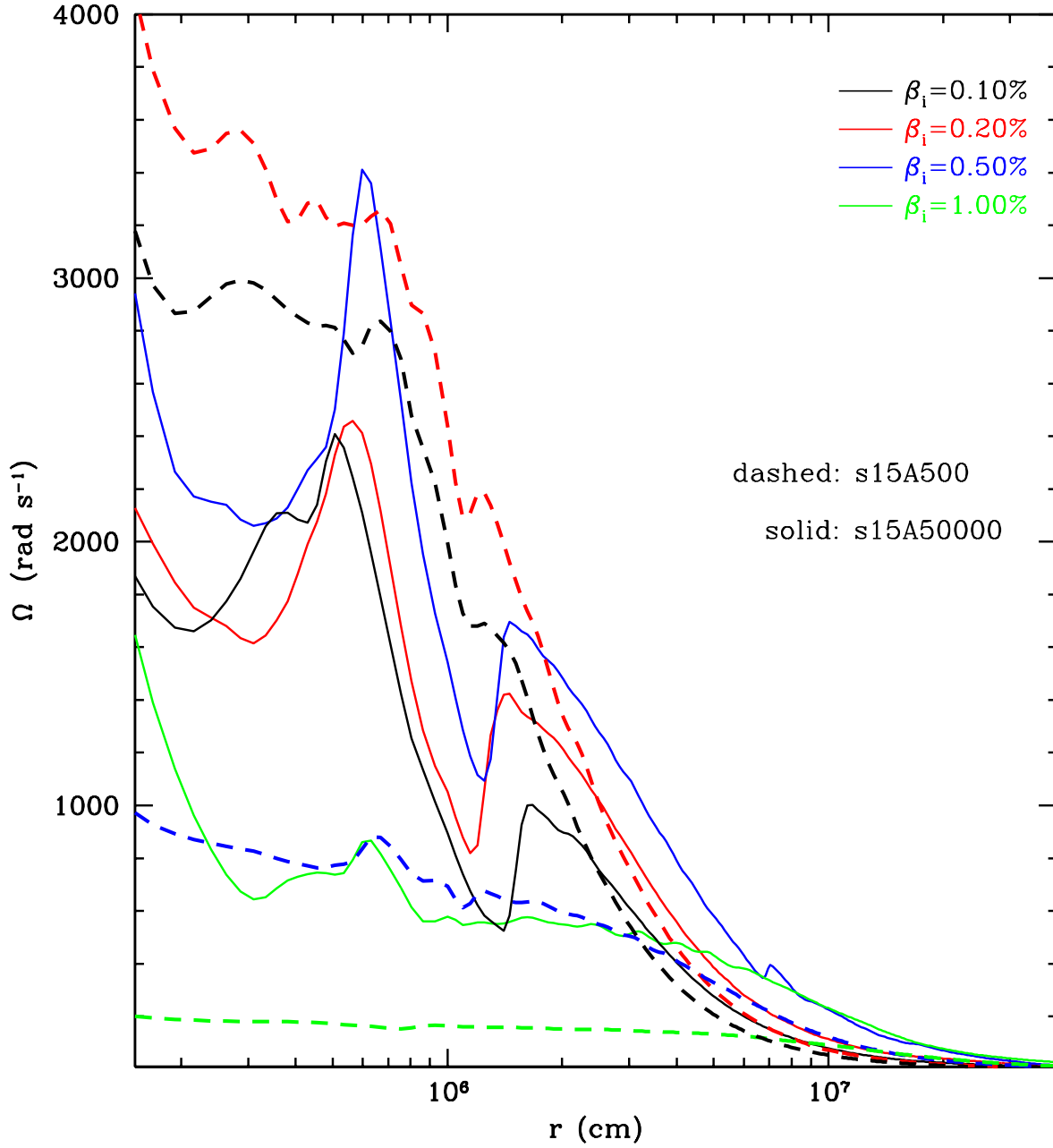
FIG. 19.— Angular velocity profiles in the equatorial region at the end of the evolution of s15 models with A=500 km (dashed) and A=50000 km (solid) and for \beta_i s of 0.10, 0.20, 0.50, and 1.00%. Interestingly, the initially rigidly rotating models ( A=50000 km) exhibit a more differentially rotating central region than the initially more differentially rotating models do. The local peak in the angular velocity at \sim 6 -8 km and the strong \Omega -gradients associated with it have been considered possible drivers of the magneto-rotational instability (MRI) (Akiyama et al. 2003).
