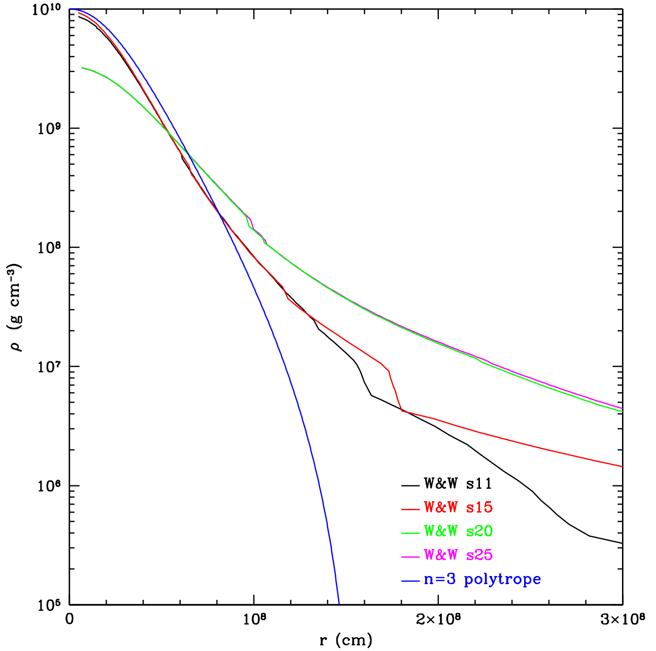
FIG. 1.— Mass density as a function of radius of the Woosley and Weaver (1995) progenitor models and the n = 3 polytropic progenitor of Zwerger and Müller (1997). Note the good correspondence in the central regions between the less massive iron cores and the polytrope, but the general disagreement at larger radii. The polytrope has a sharper edge.
