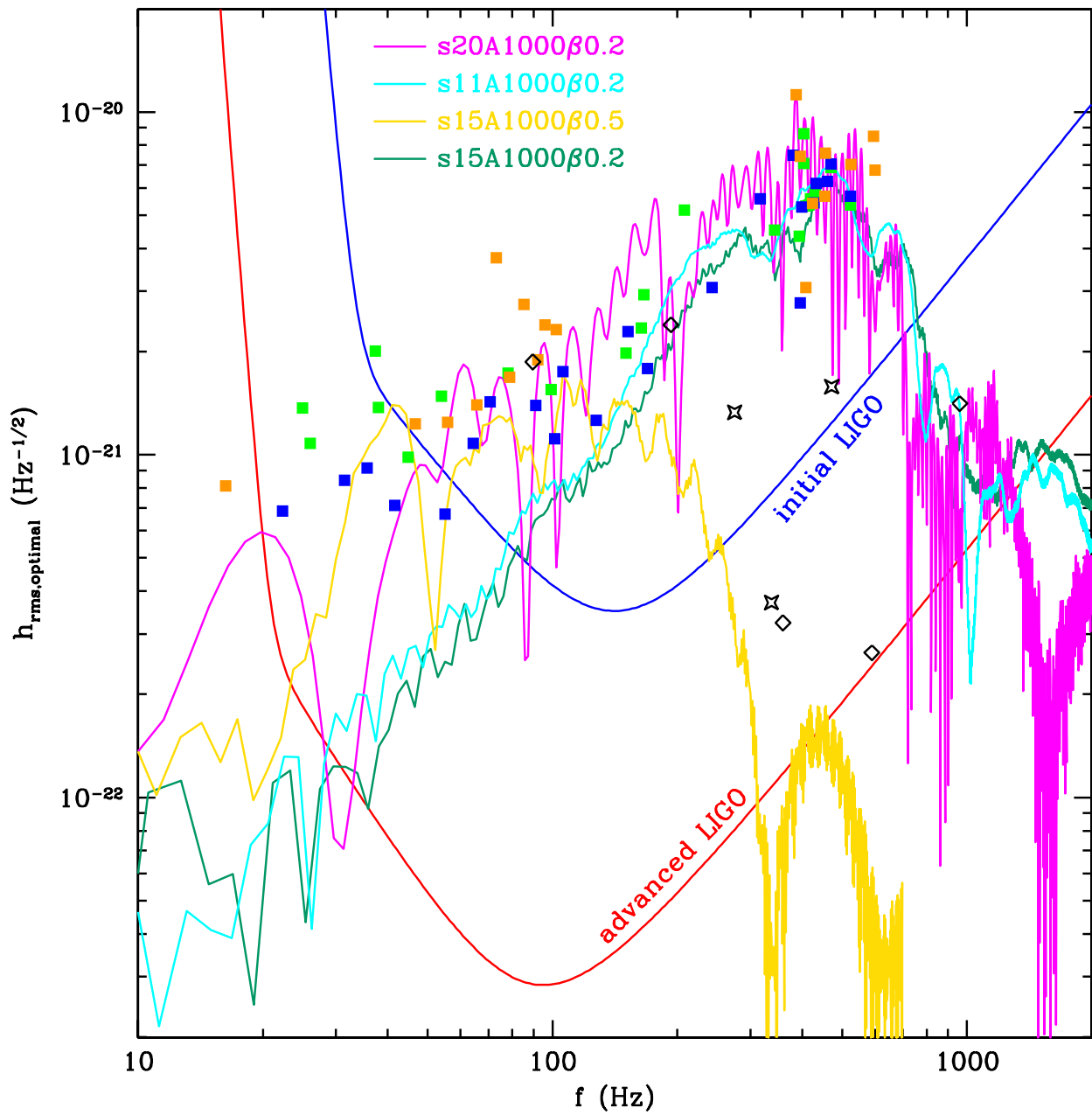
FIG. 22.— Same as Fig. 20, but with various full h_{\text{char}} spectra (using eq. 25) superposed. This plot makes clear the large width of actual spectra and the deviation from even quasi-periodic behavior of rotating collapse wave signatures.
