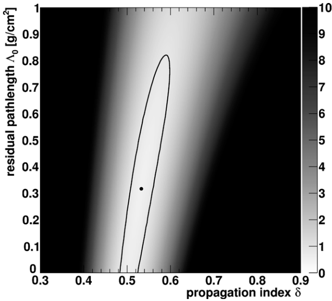
Figure 3. \chi^2 map in the parameter space of \delta vs. \Lambda_0 for the Leaky-Box model fit to TRACER data. The best-fit values are marked at (\delta, \Lambda_0) = (0.53 \pm 0.06, 0.31_{-0.31}^{+0.55} \text{ g cm}^{-2}) and the 1\sigma contour is indicated.
